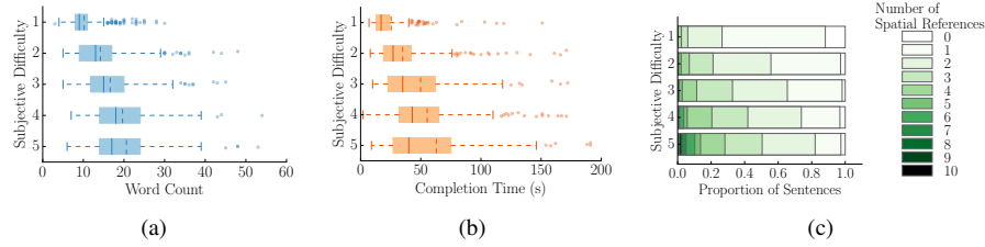
Figure 2: The effect of subjective difficulty on ratings and measures of the sentences, such as (a) word count, (b) completion time, and (c) number of spatial references.
