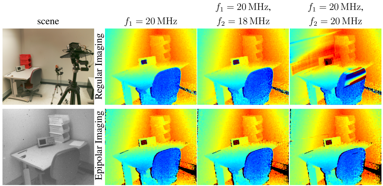
Figure 5.11: Two time-of-flight cameras are placed in a scene. When only one camera is running (second column), both regular imaging and epipolar imaging produce accurate depth maps. With both cameras operate at different frequencies (third column), the depth map with regular imaging becomes noisier because the other camera’s light source adds to the shot noise while epipolar imaging is almost unaffected. When both cameras operate at the same modulation frequency (last column), they interfere strongly in regular imaging mode. With epipolar imaging, the two cameras will usually either not interfere at all, or will interfere along a single line through the image.
