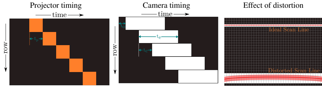
Figure 4.3: Electronic masking with a rolling shutter: At each timestep (of duration t_p ), the projector illuminates a single scanline (top left). The camera uses its rolling shutter to selectively mask pixels (top right). The masks are defined by three controllable parameters, the exposure time t_e , the time it takes the rolling shutter to read a row of pixels t_c and the offset between the projector sync output and the camera trigger input t_o . Ideally, a single projector scanline corresponds to a single camera row. In practice, because of distortion and jitter, each scanline corresponds to a band of camera pixels.
