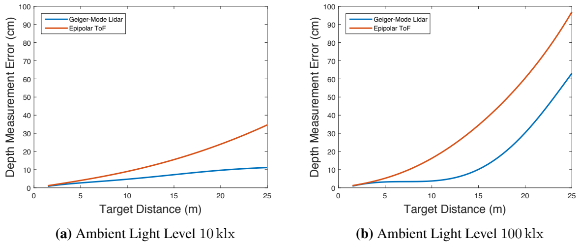
Figure 6.2: Simulated Comparisons of Epipolar CW-ToF to Geiger-Mode Lidar. For parameters of the simulated Epipolar CW-ToF camera see table 5.2. The Geiger-Mode lidar light source emits 100 pulses per depth reading, with a pulse length of 5 ns and per-pulse energy of 288 \mu J. This makes the energy emitted per depth frame equal for both sensing modalities. Field of view, operating wavelength, sensor size and other parameters were also kept equal in both simulated systems. For the simulated Geiger-Mode sensor, the photon detection probability is 0.1, the detection jitter is 100 ps and the lens aperture is set to f/4 . (a) compares the two systems under the equivalent of cloudy conditions, (b) compares the two systems under bright sunlight.
