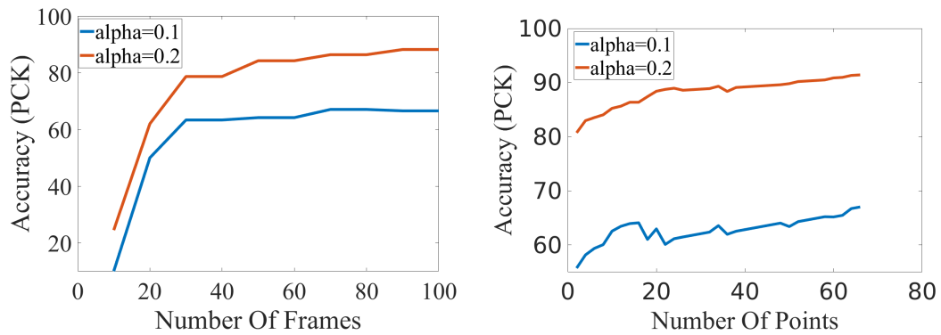
FIGURE 4.8: Analysis of accuracy with respect to increase in number of frames (left) and increase in number of unstructured points (right) used in the CarFusion algorithm.
