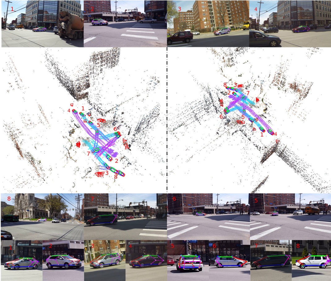
FIGURE 4.7: Visualization of the 8/43 reconstructed cars using CarFusion. We show the 2D re-projection of the reconstructions onto sample frame containing those cars. All the re-projected points fit the cars well.
