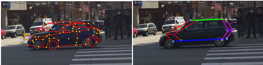
FIGURE 4.2: [Left] CAD based reconstruction [33] shows 22° angular error with respect to the motion of the vehicle. [Right] In comparison, our result shows 1° angular error. The CAD basis based methods fail due to inaccurate keypoint predictions, especially when only one side of the vehicle is visible.
