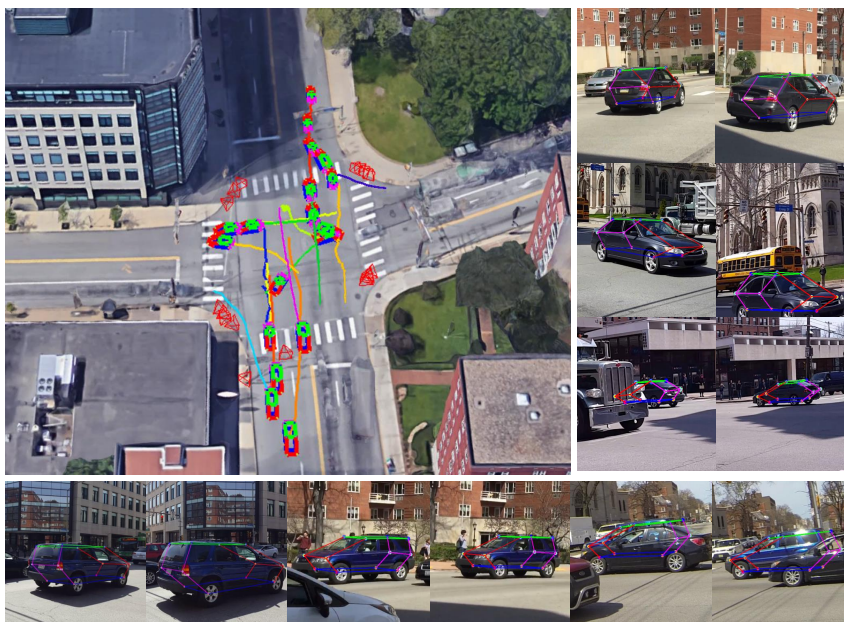
FIGURE 1.1: Reconstruction of vehicles crossing a busy intersection, making turns, going straight and changing lanes. A subset of vehicle skeletons (3D detector locations) and their 3D trajectories are augmented within the Google Earth view of the intersection. The reconstructions are reprojected into multiple views of two cars (a sedan and an SUV) demonstrating good performance under partial occlusions.
