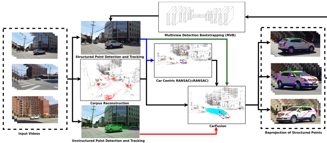
FIGURE 1.2: CarFusion: Our overall pipeline for dynamic 3D reconstruction of multiple cars from uncalibrated and unsynchronized video cameras. We fuse the structured points (detected vehicle parts) and the tracks of the unstructured feature points to obtain precise reconstruction of the moving vehicle. The reconstructions are reprojected into all the views and are used to bootstrap and improve the detectors.
