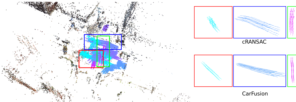
FIGURE 4.4: Visualization of the reconstructed trajectories of multiple cars using cRANSAC. The insets on the right show detailed comparisons of the trajectories stability between cRANSAC and CarFusion. CarFusion produces clearly more stable trajectories. Visually, they correspond well to the motion of a moving car.
