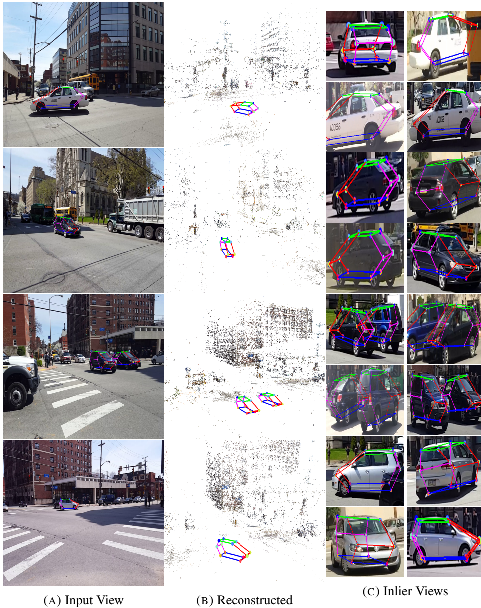
FIGURE 4.6: We show the fitting of vehicles using our Multi-view RANSAC based object fitting
