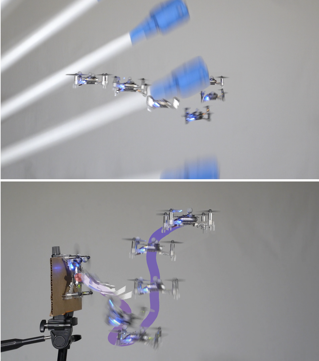
Figure 3.1: TinyMPC is a fast convex model predictive control solver that enables real-time optimal control on resource-constrained microcontrollers. We demonstrate its efficacy in dynamic obstacle avoidance (top) and recovery from 90^\circ attitude errors (bottom) on a 27 gram Crazyflie quadrotor.
