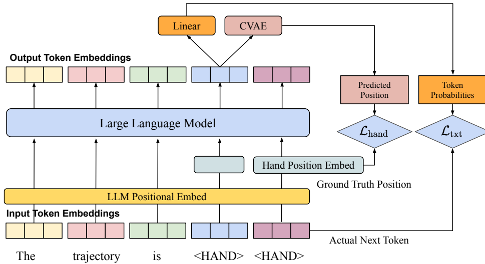
Figure A.1: Illustration of training pipeline.
