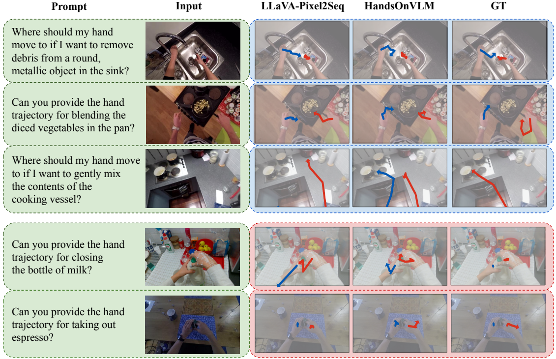
Figure 5.1: Qualitative results for different samples from the validation split of our RBHP dataset (top in blue) and zero-shot evaluations on completely unseen datasets FPHA and H2O (bottom in pink). The left-hand trajectory is visualized in blue and the right-hand trajectory is in red. The arrows denote the direction of each trajectory. GT trajectories are provided for reference.
