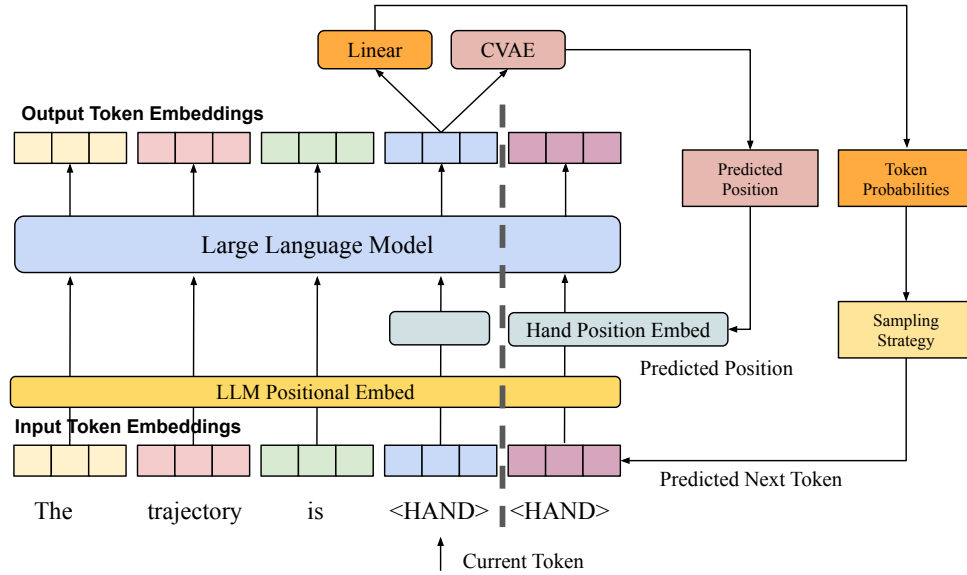
Figure A.2: Illustration of inference pipeline.
