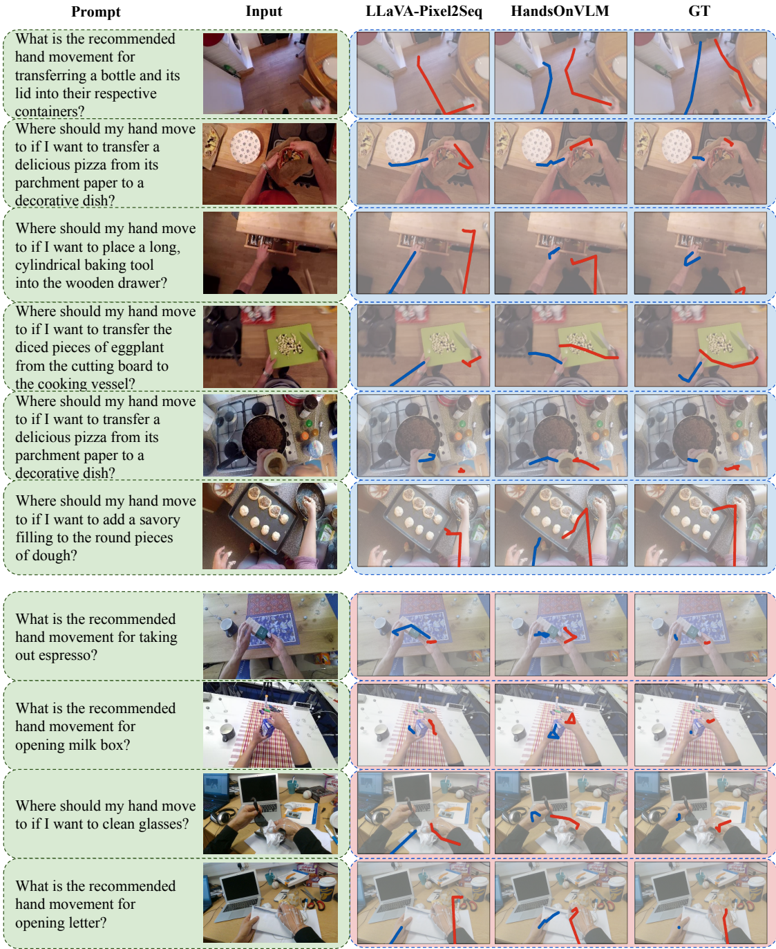
Figure A.6: More Qualitative results for different samples from the validation split of our RBHP dataset (top in blue) and zero-shot evaluations on completely unseen datasets FPHA and H2O (bottom in pink). GT trajectories are provided for reference.
