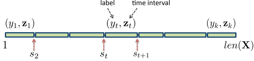
FIGURE 4.2: Joint segmentation and recognition process – we need to find the events' boundary points s_1, \dots, s_{k+1} and the class labels y_1, \dots, y_k .
