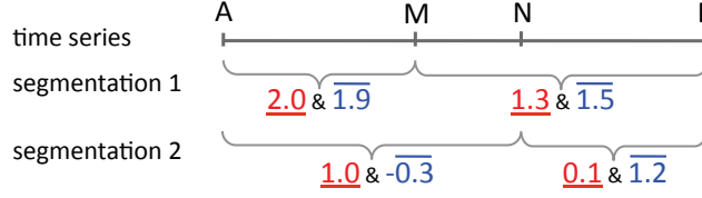
FIGURE 4.1: Which segmentation is preferred, breaking time series AB at M or N ? Suppose there are only two classes, SVM scores of the first and second class for corresponding segments are printed in red and blue, respectively. Our segmentation criterion prefers to cut at N because the resulting segments can be confidently classified. This figure is best seen in color.
