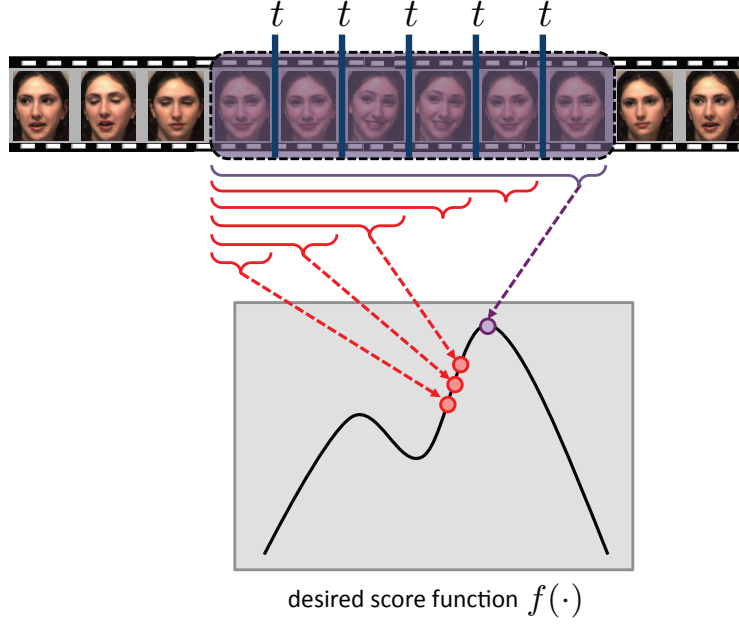
FIGURE 5.4: Monotonicity requirement – the detection score (confidence) of a partial event cannot exceed the score of an encompassing partial event. MMED provides a principled mechanism to achieve this monotonicity.
