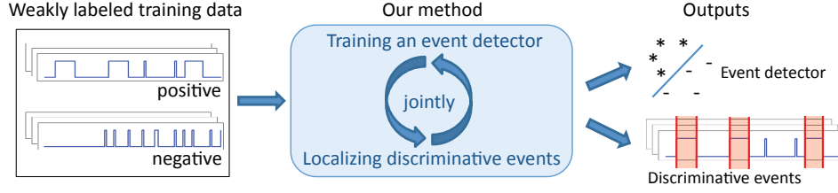
FIGURE 6.1: A framework for simultaneous localization of discriminative events and training a detector to detect them.
