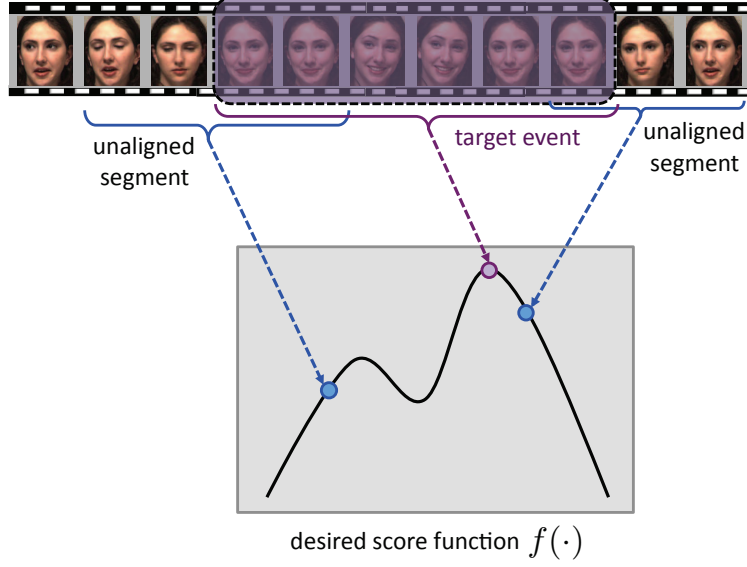
FIGURE 3.1: Desired detection function – the target event must have the highest detection score. During training, we learn the detection function by enforcing this constraint.
