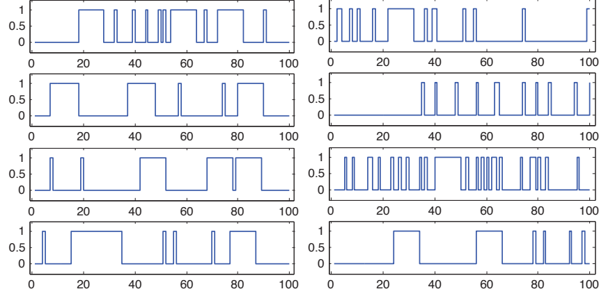
FIGURE 6.2: What distinguishes the time series on the left from the ones on the right? Left: positive examples, each containing three long segments with value 1 at random locations. Right: negative examples, each containing fewer than three long segments with value 1. All signals are perturbed with measurement noise corresponding to spikes with value 1 at random locations.
