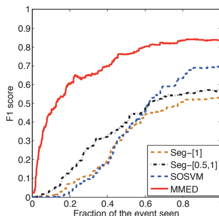
FIGURE 5.8: F1-score curves on Weizmann dataset; MMED provides better localization for the event of interest, especially when the fraction of the event observed is small. This figure is best seen in color.
