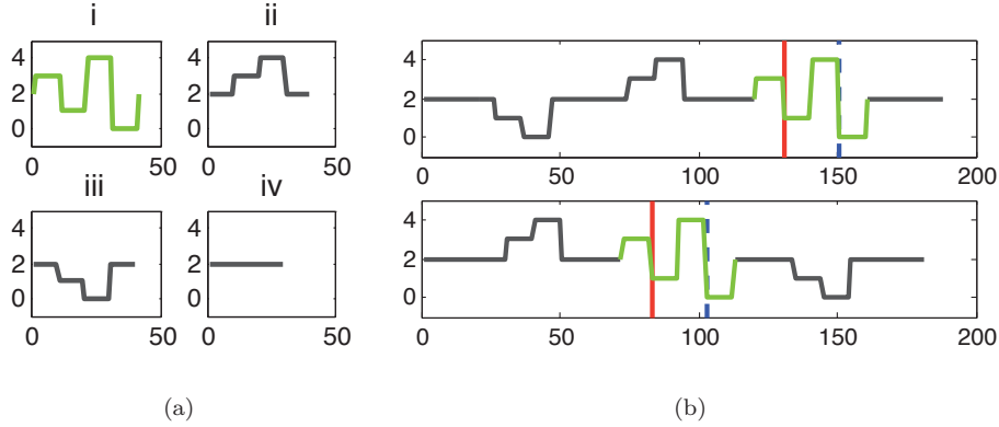
FIGURE 5.5: Synthetic data experiment. (a): time series were created by concatenating the event of interest (i) and several instances of other events (ii)–(iv). (b): examples of testing time series; the solid vertical red lines mark the moments that our method starts to detect the happening of the event of interest while the dash blue lines are the results of SOSVM. This figure is best seen in color.
