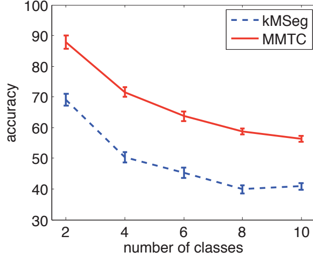
FIGURE 7.2: Segmentation-clustering accuracy as a function of the number of classes. MMTC outperforms kMSeg.
