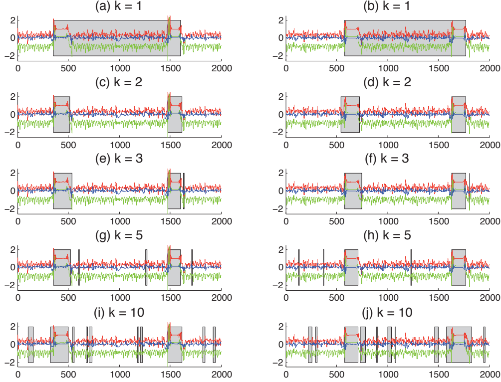
FIGURE 6.5: Discriminative localization in human motion analysis. This figure shows two examples of testing time series and the results for different values of \bar{k} , the number of segments in \bar{k} -segmentations. The left sub-figures (a, c, e, g, i) show the same time series, while the right subfigures (b, d, f, h, j) depict another time series. \bar{k} is 1, 2, 3, 5, 10 for (a, b), (c, d), (e, f), (g, h), and (i, j) respectively. Our method successfully discovers the discriminative patterns (falling events) for a wide range of \bar{k} values.
