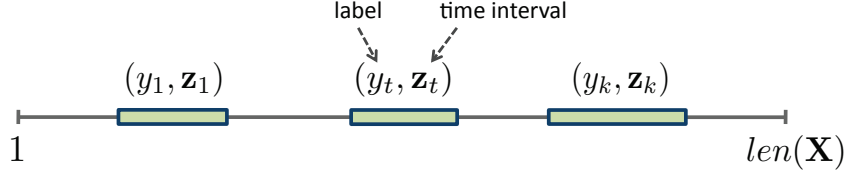
FIGURE 2.1: The common goal of our time series analysis problems – to factorize a time series into a set of non-overlapping segments and assign a class/cluster label to some or all segments. y_t \in \{1, \dots, m\} is a class/cluster label, and \mathbf{z}_t consists of two scalars for the start and the end of an event.
