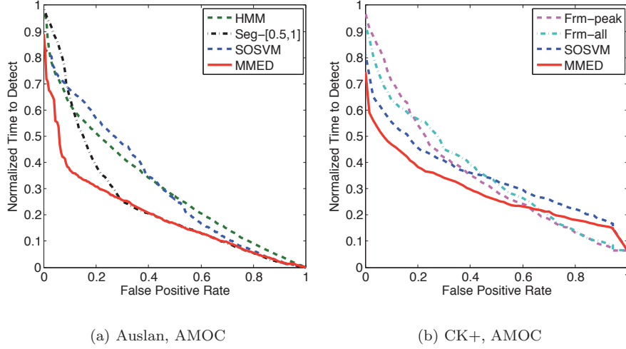
FIGURE 5.6: AMOC curves on Auslan and CK+ datasets; at the same false positive rate, MMED detects target events sooner than the other methods. This figure is best seen in color.
