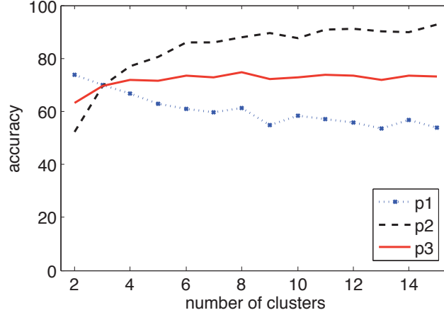
FIGURE 7.3: Sensitivity analysis – accuracy values when the desired number of clusters varies around 10, the true number of classes.
