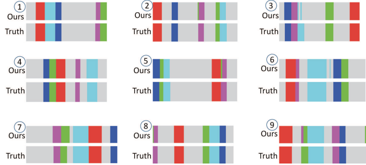
FIGURE 4.7: Automatic segmentation-recognition versus human-labeled ground truth for Weizmann dataset. The segments are color coded; red, cyan, magenta, blue, green, and gray correspond to bend , jack , jump , pjump , run , and null classes, respectively. This figure is best seen in color.
