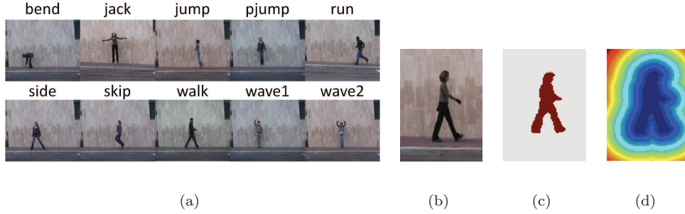
FIGURE 4.6: Weizmann dataset. (a): typical frames. (b)-(d): how frame-level features are computed; (b) is an original frame, (c) is the binary mask, and (d) is the Euclidean distance transform.
