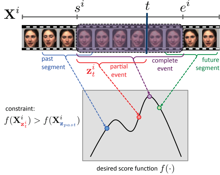
FIGURE 5.2: From desire to constraint. The desired score function for early event detection: the complete event must have highest detection score, and the detection score of a partial event must be bigger than that of any segment that ends before the partial event. To learn this function, we explicitly consider partial events during training. At time t , the score of the truncated event (red segment) is required to be bigger than the score of any segment in the past (e.g., blue segment); however, it is not required to be bigger than the score of any future segment (e.g., green segment). This figure is best seen in color.
