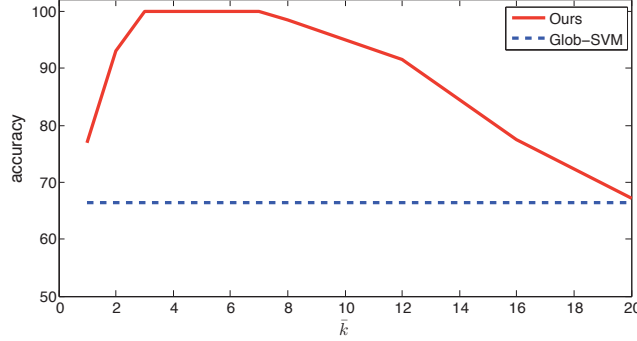
FIGURE 6.3: Classification performance on synthetic time series. For our method, we show the accuracy obtained using different values of \bar{k} , the maximum number of discriminative time intervals allowed. Here Glob-SVM , traditional SVM based on the global statistics of the signals, yields an accuracy rate of 66.5%, which does not depend on \bar{k}
