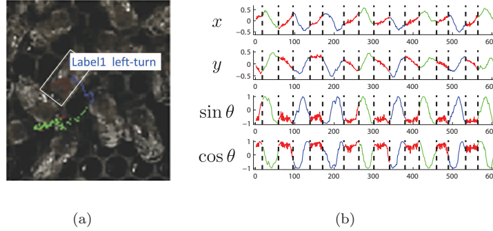
FIGURE 4.4: a) Visual tracking: green + blue trajectory and the bounding box for tracking. b) plots of the frame-level features [x, y, \sin(\theta), \cos(\theta)] . Red, green, and blue correspond to waggle, right-turn, and left-turn, respectively. This is best seen in color.
