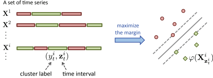
FIGURE 7.1: Temporal clustering: time series are partitioned into segments \{z_t^i\} and similar segments are grouped into classes (i.e., assigning a cluster label y_t^i to each segment z_t^i ). The objective is to maximize the margin for the separation between clusters. Though this figure only illustrates the case of two classes, our method is multi-class.
