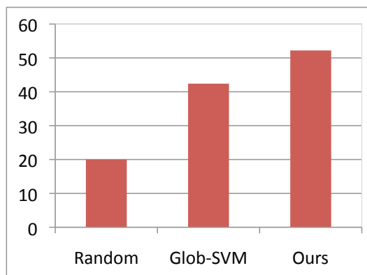
FIGURE 6.8: The mean accuracies on CMU-MMAC dataset – our method significantly outperforms Glob-SVM.
