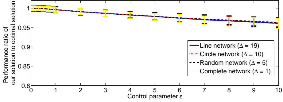
Figure 4.8: Total payoffs of assignment by our algorithm for different robot network diameter \Delta . We generate 100 samples for each different \epsilon .
