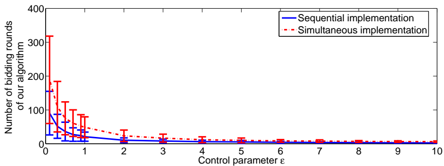
Figure 4.5: Number of bidding rounds of our algorithm as a function of parameter \epsilon . The solid (dashed) line shows the number of rounds for the sequential (simultaneous) implementation of our algorithm to terminate.
