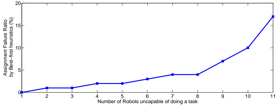
Figure 4.15: Assignment failure ratio as a function of number of robots incapable of doing a task. n_r = 20
