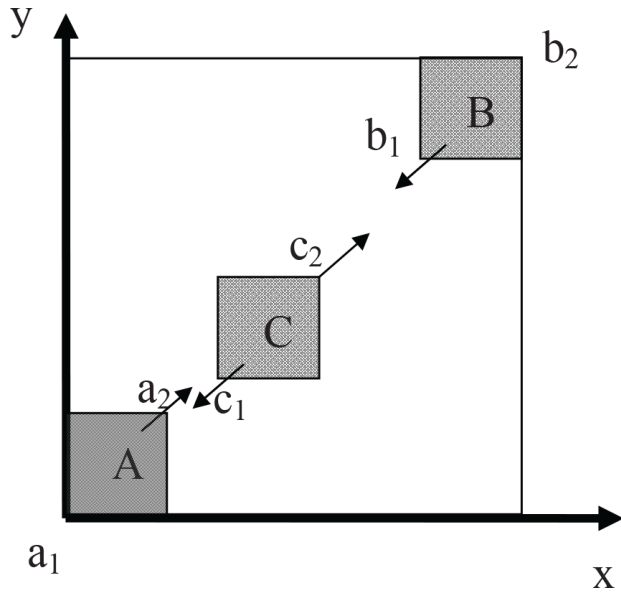
Figure 9.2: The illustration of how we generate the payoffs between robots and tasks. The coordinates of end points of A : a_1 = (0,0) , a_2 = (u,u) ; B : b_1 = (10 - u, 10 - u) , b_2 = (10,10) ; C : c_1 = (4.5 - 0.45u, 4.5 - 0.45u) , c_2 = (4.5 + 0.55u, 4.5 + 0.55u) . When u = 10 , A , B and C would become the whole 10 \times 10 square. The arrows represent the expanding directions of the square A, B, C with parameter u increasing.
