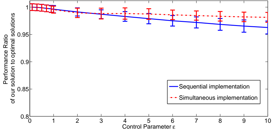
Figure 4.4: Total payoffs of assignment by our algorithm as a function of parameter \epsilon , which is the minimum possible price increase during the bidding procedure. The optimal solution can be achieved when we set \epsilon < \frac{\text{min\_diff}}{\sum_{i=1}^{n_r} N_i} where \text{min\_diff} is the minimum difference between any two individual payoffs a_{ij} .
