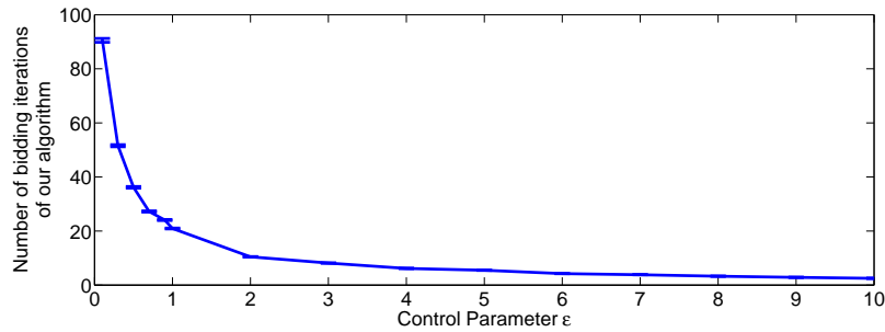
Figure 5.3: Convergence time of our algorithm as a function of \epsilon . The figure shows the number of rounds for our algorithm to terminate, where one round means all robots sequentially implement Algorithm 2 for one iteration.
