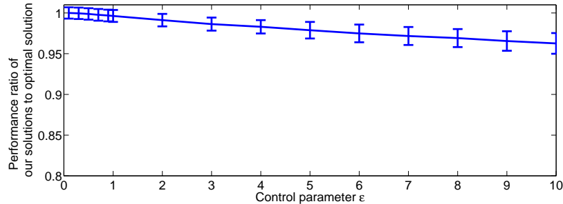
Figure 5.2: Performance ratio of our solution to the optimal one as a function of \epsilon , which is the minimum price increase for new bids. The optimal solution can be achieved when we set \epsilon < \frac{\min\_diff}{\sum_{i=1}^{n_r} N_i} where \min\_diff is the minimum difference between any two individual payoffs a_{ij} .
