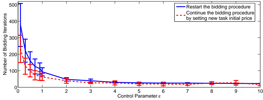
Figure 4.13: Number of bidding iterations of our algorithm as a function of parameter \epsilon for dynamically arising tasks. The solid line shows the number of iterations for the approach of restarting the whole procedure. The dashed line shows the number of iterations for the approach of continuing the bidding procedure with new task initial price set as in Section 4.6.3.
