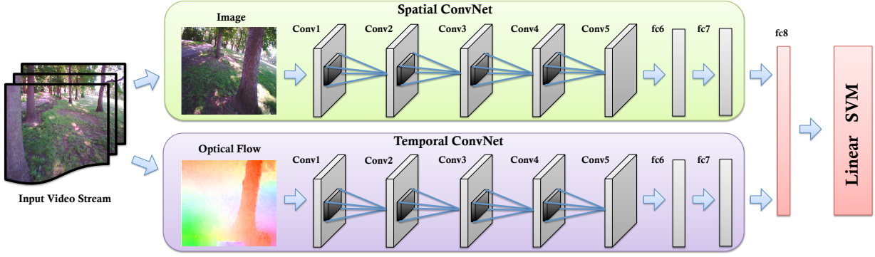
Figure 3.2: Spatio-temporal convolutional neural net architecture for deep introspective perception. The layer schematics are same as AlexNet [53]
