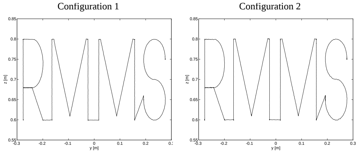
Figure 2-11a. measured path (solid) and desired path (dotted).
