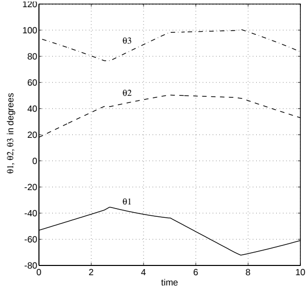
Figure 4-7. Fault tolerant trajectories for the individual joints.
