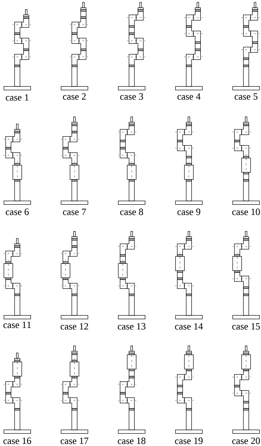
Figure 6-3. Different module orders for 3-DOF manipulators. Each of these cases represents a group of designs obtained by cycling through all the possible combinations of relative orientations. (512 combinations for cases 1–4; 64 combinations for the other cases)
