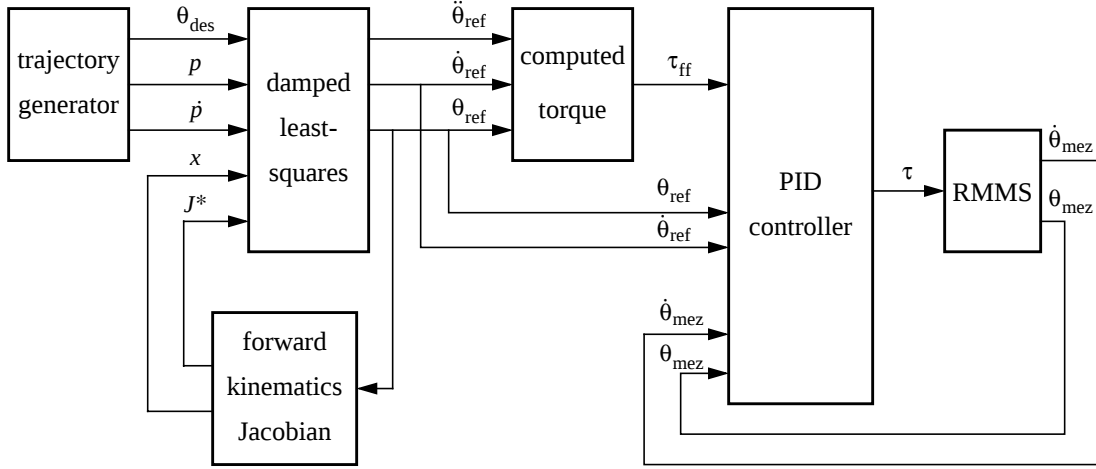
Figure 5-2. The control structure of the RMMS
