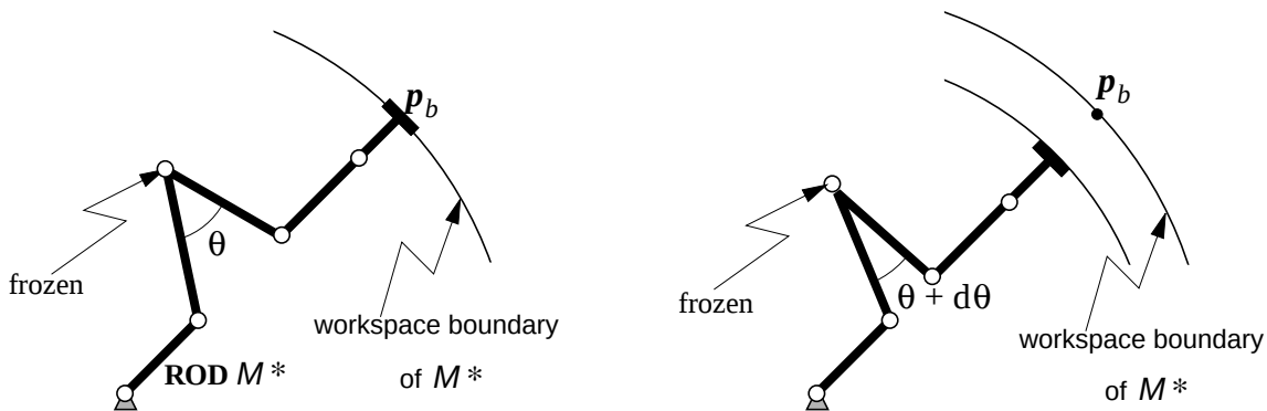
Figure 3-3. A ROD unable to reach a point outside the FTWS.
