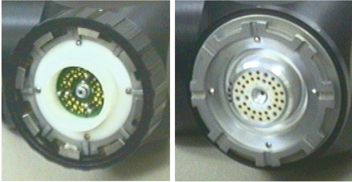
Figure 2-4. A male and female RMMS connector.
