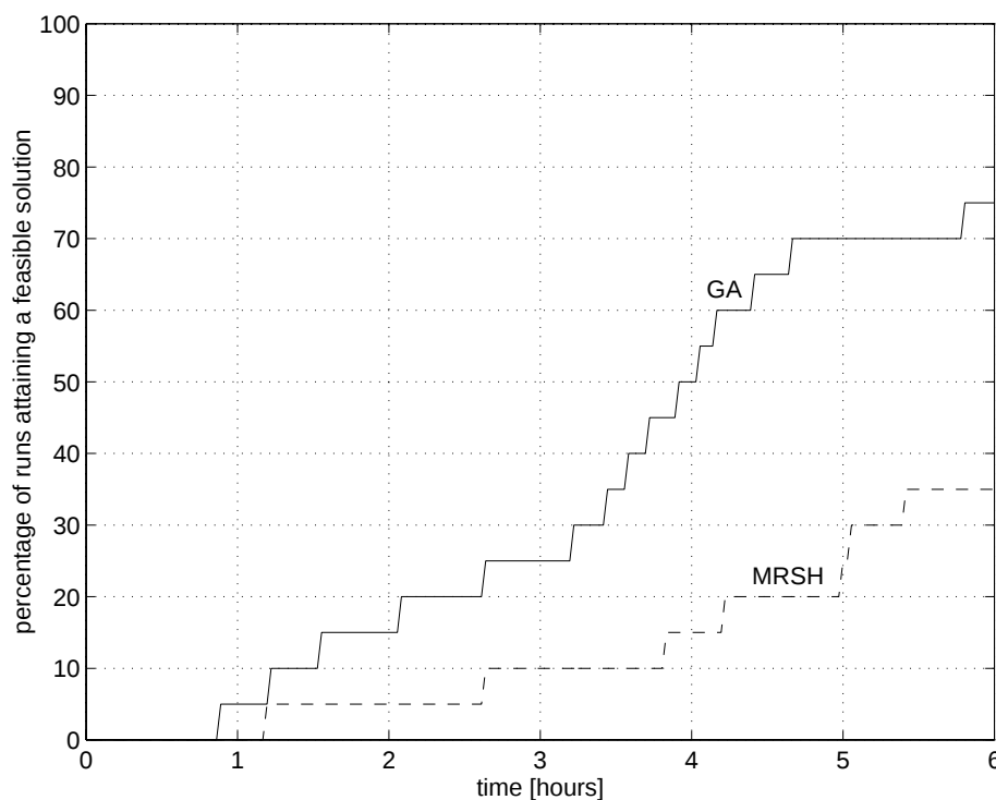
Figure 7-4. Percentage of the runs attaining a feasible solution.
