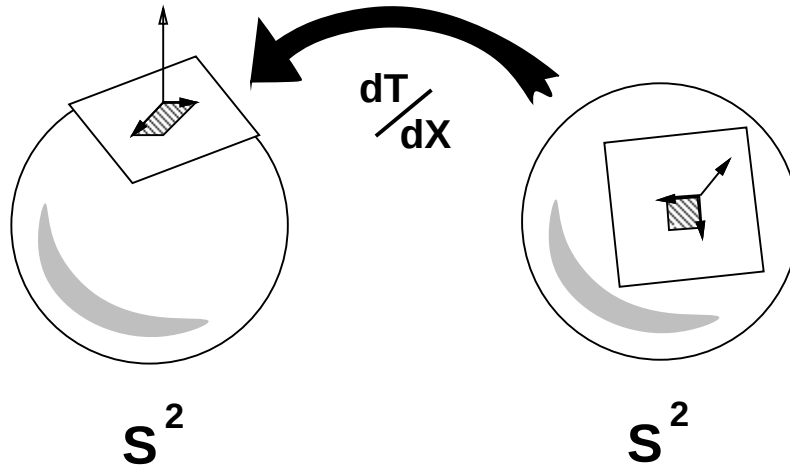
Figure C.3: The Jacobian of a transformation T from S^2 to S^2 . The Jacobian matrix \partial T / \partial X maps a unit square in the tangent plane at point x_0 on S^2 into a parallelogram in the tangent plane at point T(x_0) on S^2 . The change in area between the unit square and the tangent parallelogram is the Jacobian of transformation T at point x_0 .
