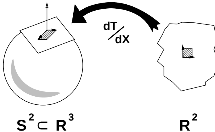
Figure C.2: The Jacobian of a transformation T from R^2 to S^2 . The Jacobian matrix \partial T / \partial X maps a unit square at point x_0 into a parallelogram in the tangent plane at point T(x_0) on S^2 . The change in area between the unit square and the tangent parallelogram is the Jacobian of transformation T at point x_0 .
