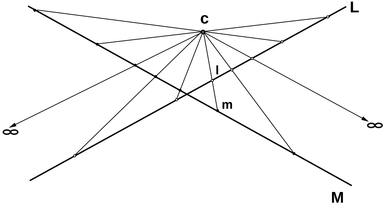
Figure A.1: A perspectivity between two lines in a plane.
