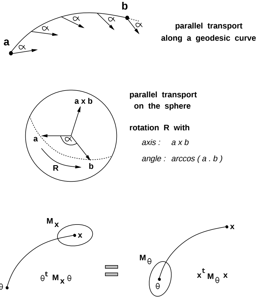
Figure 3.5: Parallel transport on the sphere. Parallel transport provides a general mechanism for “translating” vectors on the surface of the sphere. Transport from point a to b is achieved by performing the minimal rotation taking a to point b . The likelihood value computed by performing parallel transport of a Bingham density function from x_i to \theta , then evaluating the probability at point x_i , is the same as the value returned by the original density function centered around x_i , when evaluated at point \theta .
