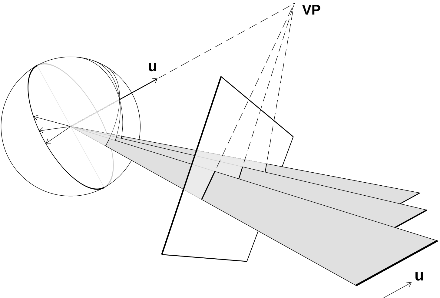
Figure 2.1: Vanishing point geometry.
