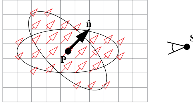
Figure 10: The insertion of a point in to the surface probability field. Vectors aligned with the point's surface normal with magnitude depending on the sum of the Point Spread and Sensor Error Model are inserted into the voxel space. S is the sensor origin.
