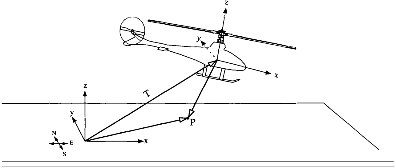
Figure 2-3 Helicopter and Ground Frames and Transformations
