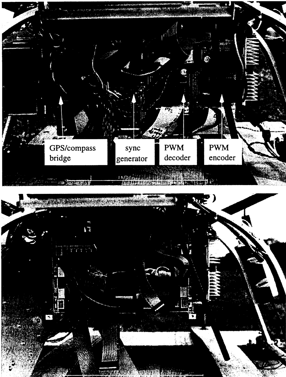
Figure 5-8. On-board Computing
