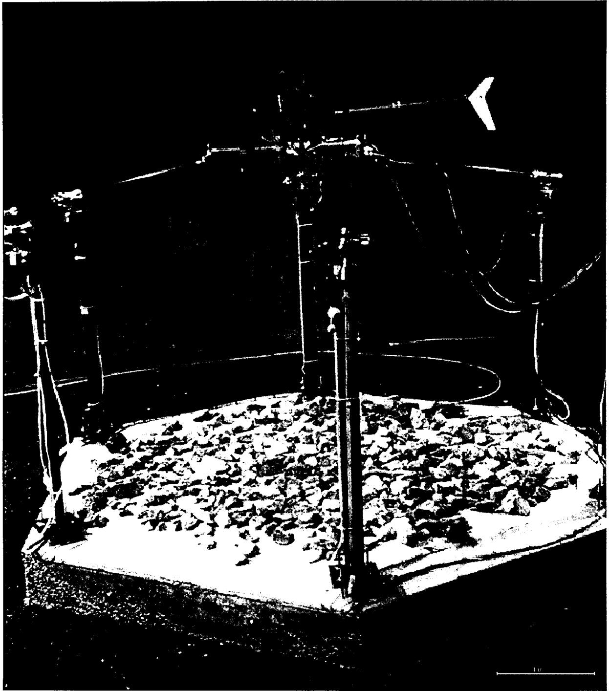
Figure 2-14 6-DOF Testbed for Indoor Position Estimation Experiments
