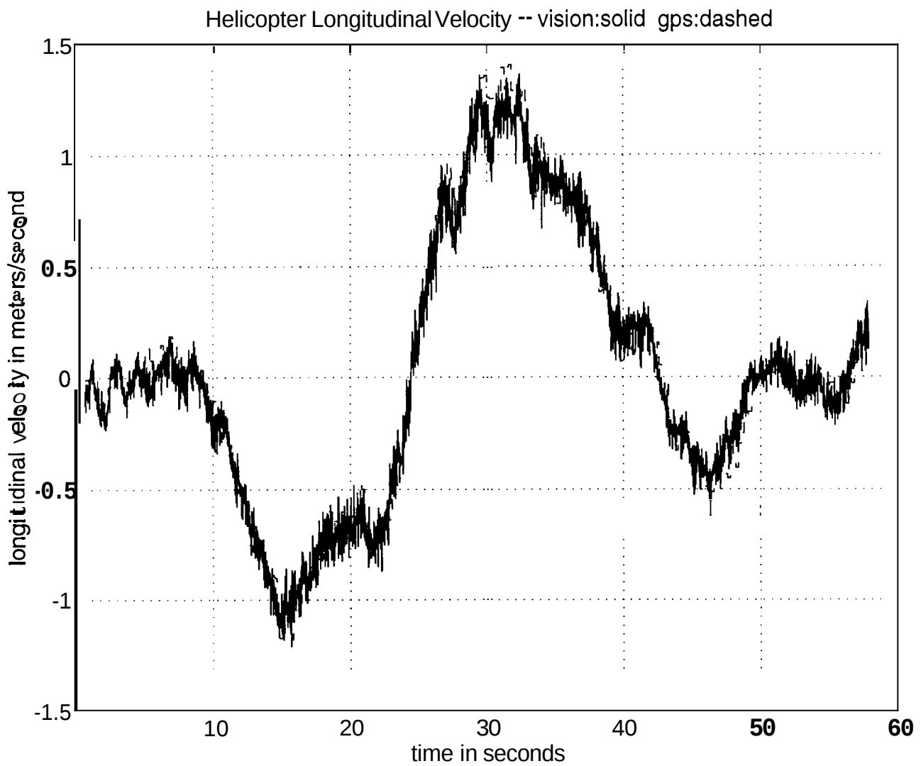
Figure 5-21. Longitudinal velocity
