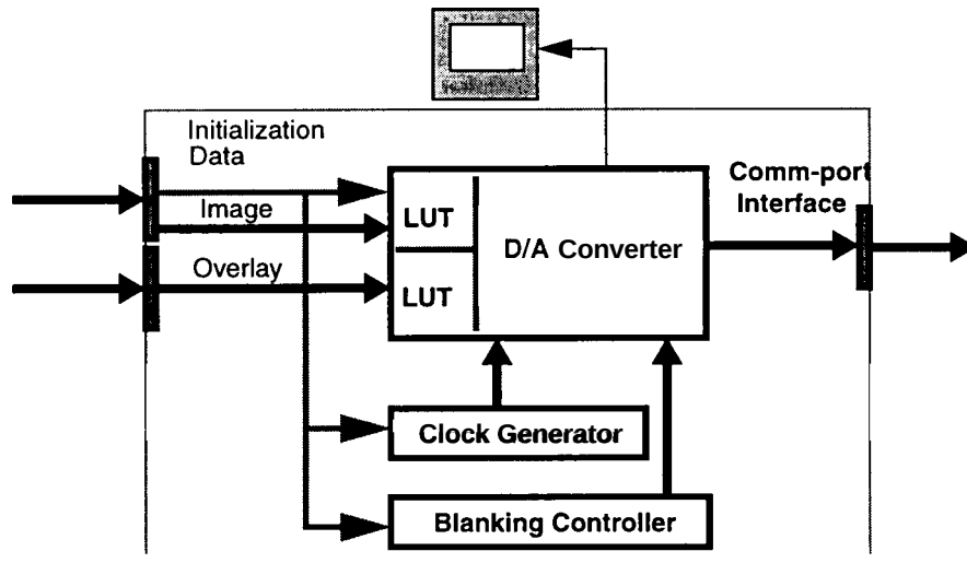
Figure 3-5 D/A Module Structure
