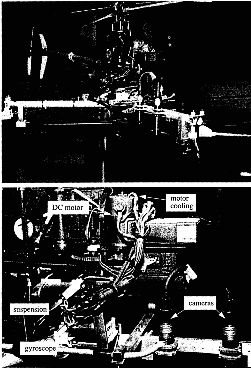
Figure A-2. 6-DOF testbed helicopter
