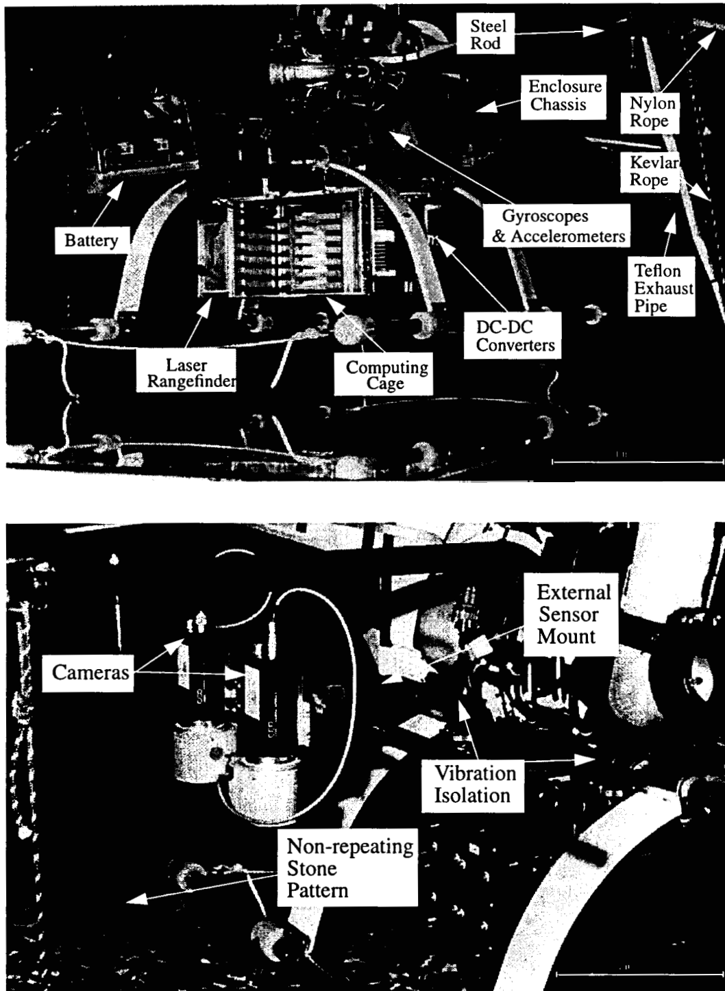
Figure 4-4. Testbed R50 helicopter
