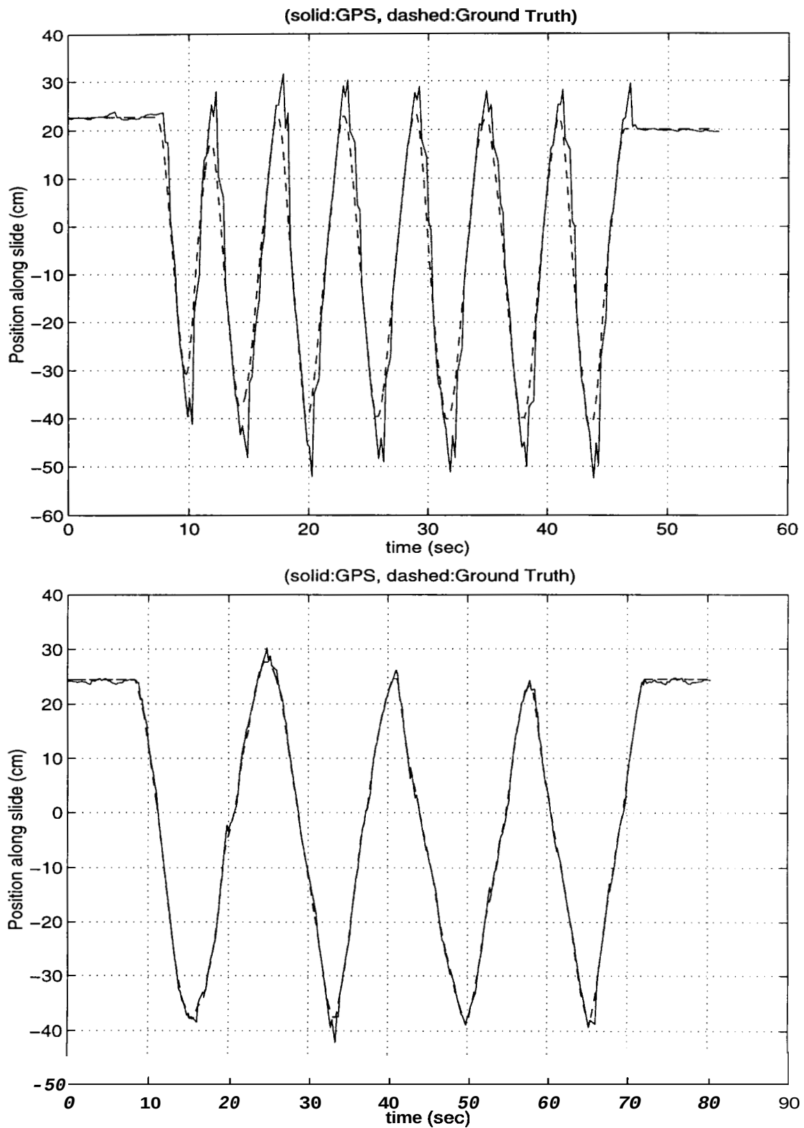
Figure 5-3. Carrier Phase DGPS Performance
