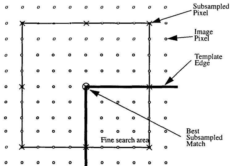
Figure 2-12 Coarse-to-fine search
