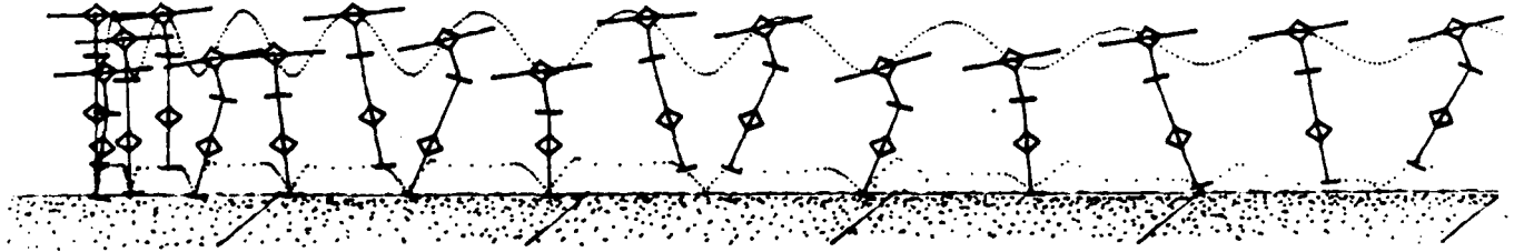
Figure 6-13: Cartoon of running controlled by leg sweeping algorithm. Model accelerates from standing start to about 2.2 m/sec in 10 sec. The dotted lines represent the paths of hip and foot. (20 msec/dot, .6 sec/stick figure.) Maximum speed is limited by clearance between foot and ground. When the stride becomes too long the model stubs its toe .
