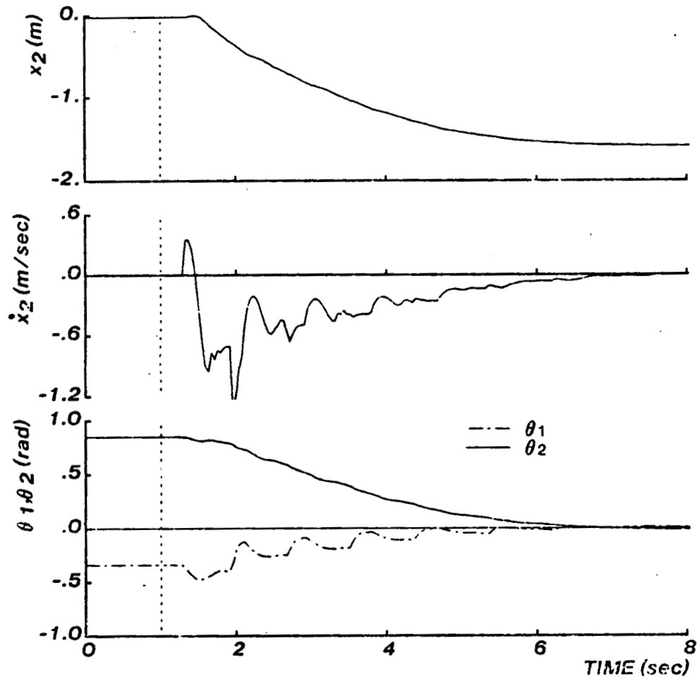
Figure 5-2: Orientation of the body is corrected using tabular method. At t=0 initial error in body attitude was 0.8 radians. At t=1 gravity is turned on and hopping begins. State errors approached zero about 6 sec later. Horizontal position is not controlled, so position changes without correction. ( Q_1=1.5, Q_2=5.0, Q_3=1.0 )
