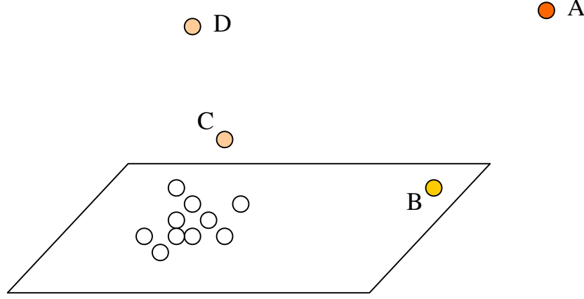
Figure 4.1: Structure outliers and extreme outliers. The 3-dimensional data points reside in a 2-dimensional subspace. Point A, B, and D are extreme outliers, but B is in the subspace. Point C is a structure outlier.
