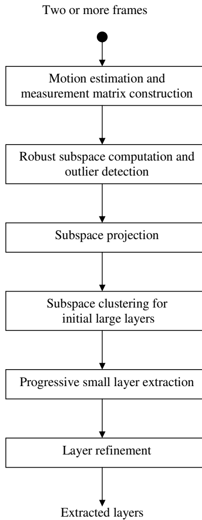
Figure 5.1: The procedure of layer extraction algorithm.
