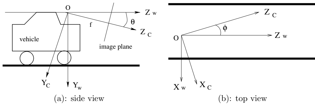
Figure 7.8: Coordinate frames.
