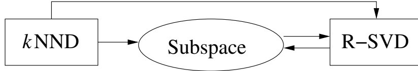
Figure 4.2: Three integrated components in our layer extraction algorithm. Subspace is the core component.
